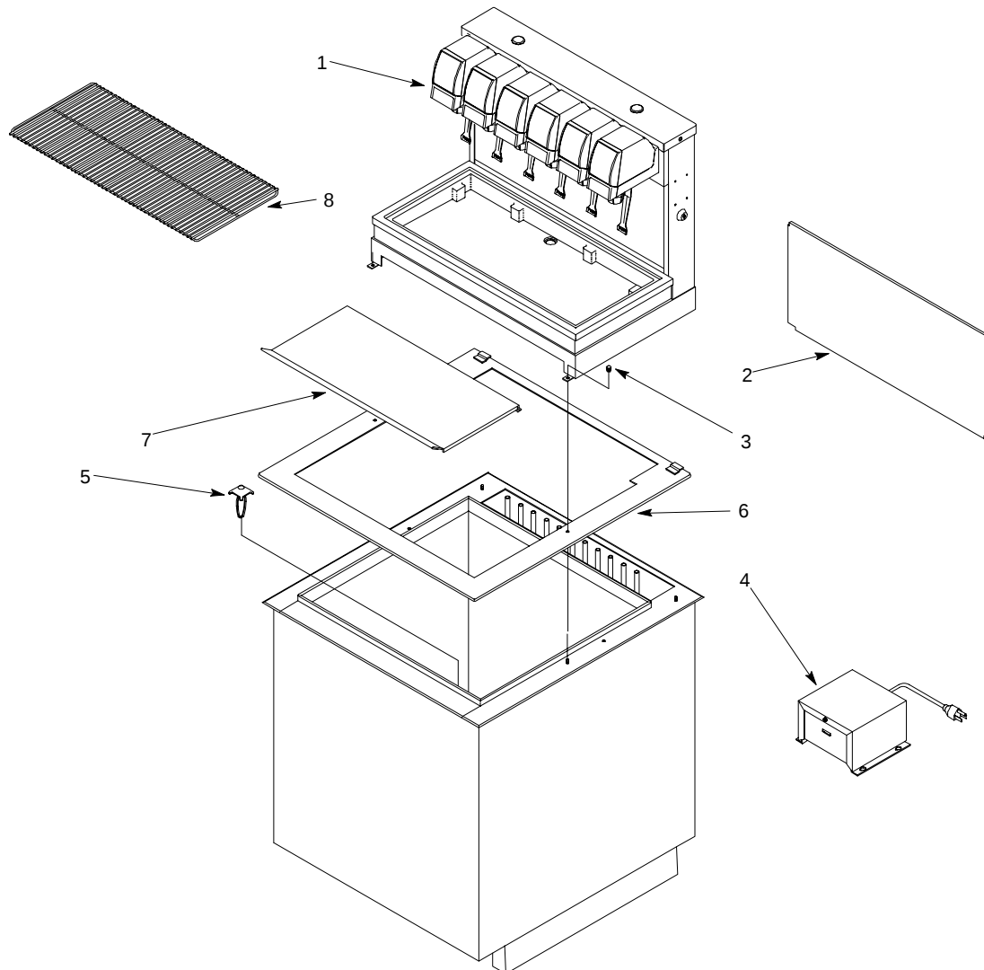
FIGURE 1. CB2323 L ASSEMBLY
