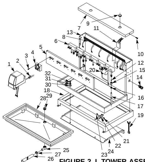
FIGURE 2. L TOWER ASSEMBLY
