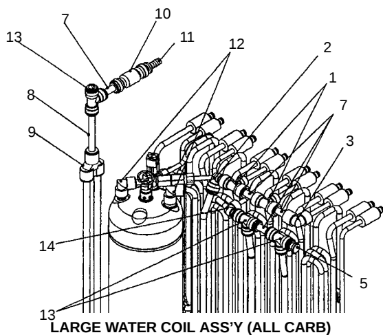
LARGE WATER COIL ASS'Y (ALL CARB)
