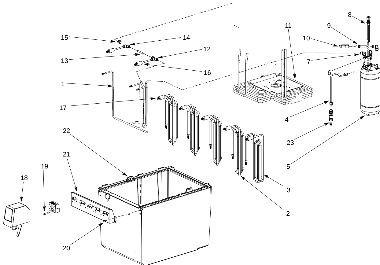
FIGURE 4. COIL AND DISPENSING VALVE COMPONENTS
