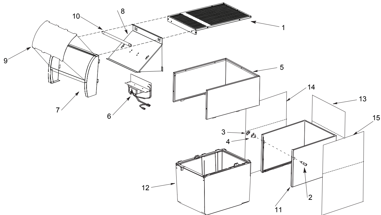
FIGURE 2. HOOD AND PANEL COMPONENTS
