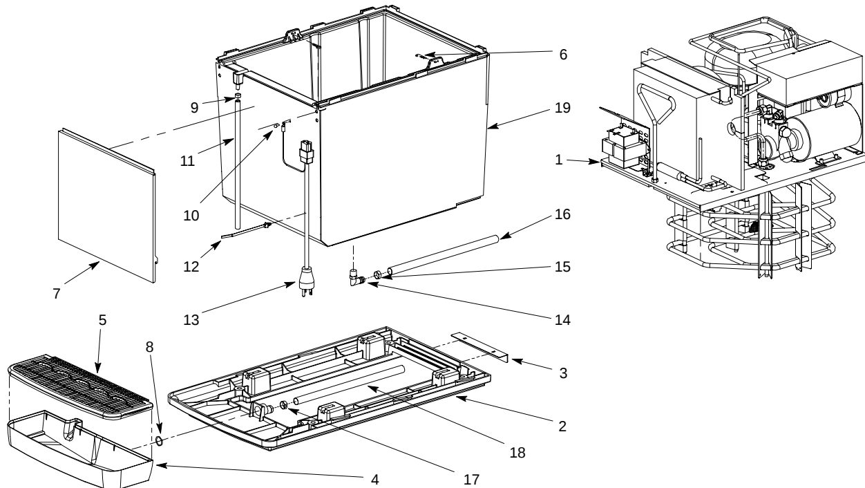
FIGURE 3. WATER BATH COMPONENTS
