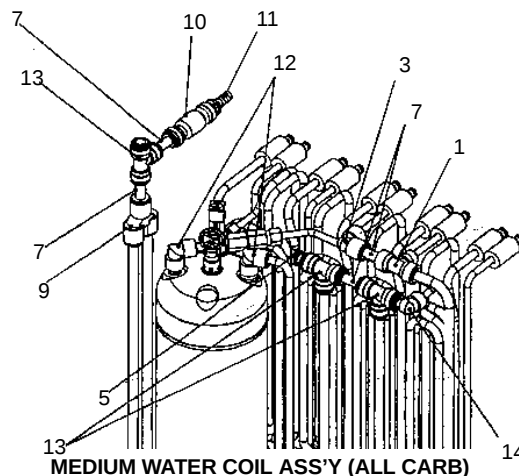
MEDIUM WATER COIL ASS'Y (ALL CARB)
