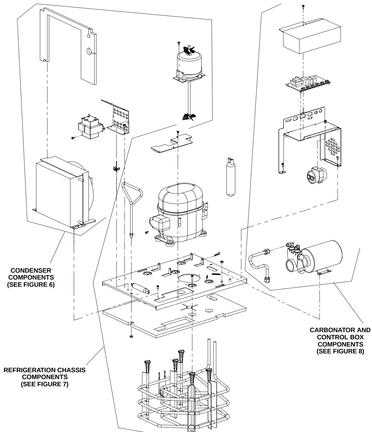
FIGURE 5. REFRIGERATION ASSEMBLY
