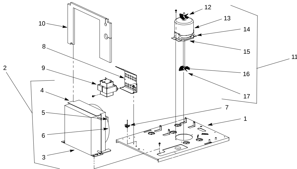
FIGURE 6. CONDENSER COMPONENTS
