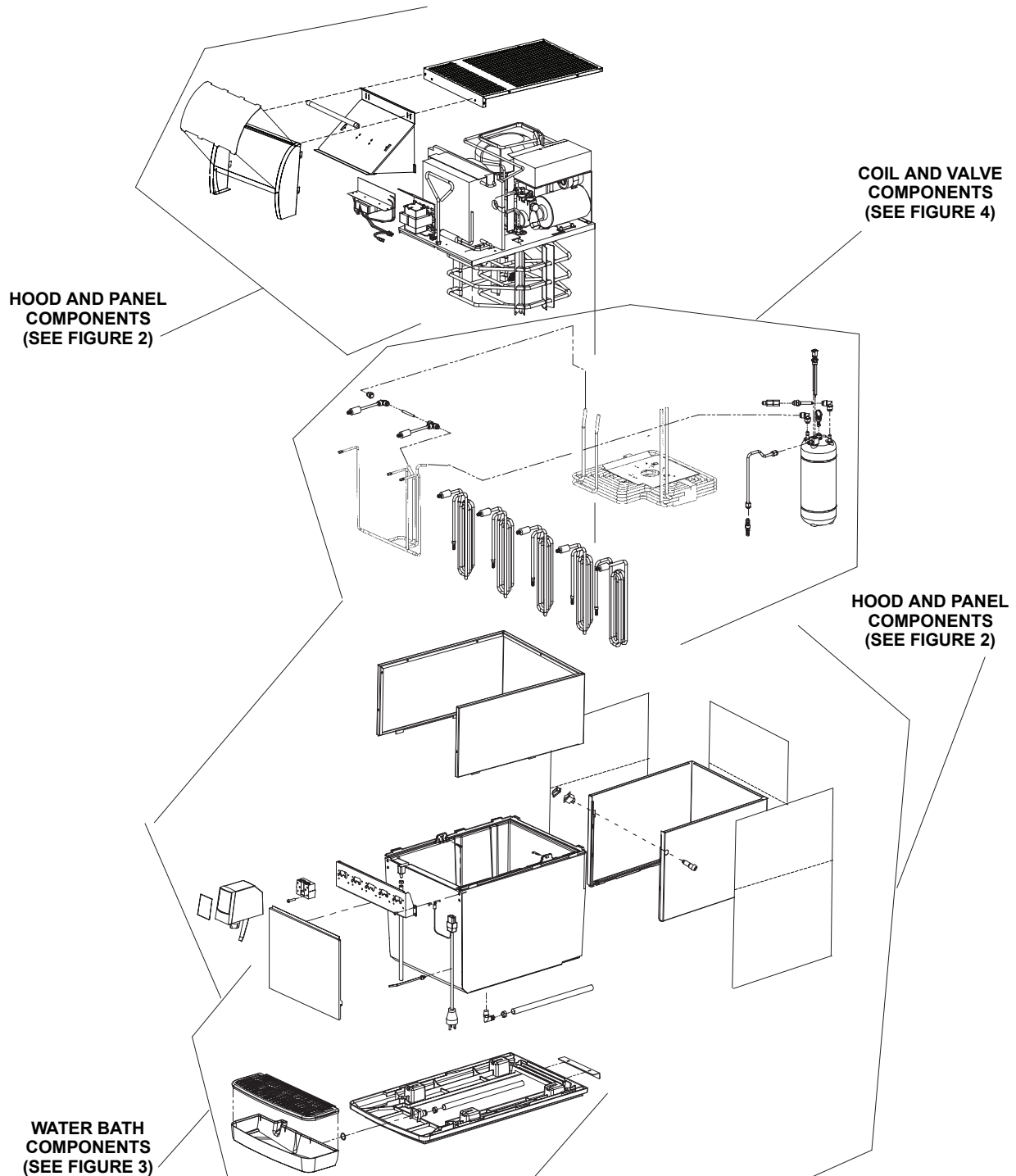
FIGURE 1. OLYMPUS GENERAL ASSEMBLY
