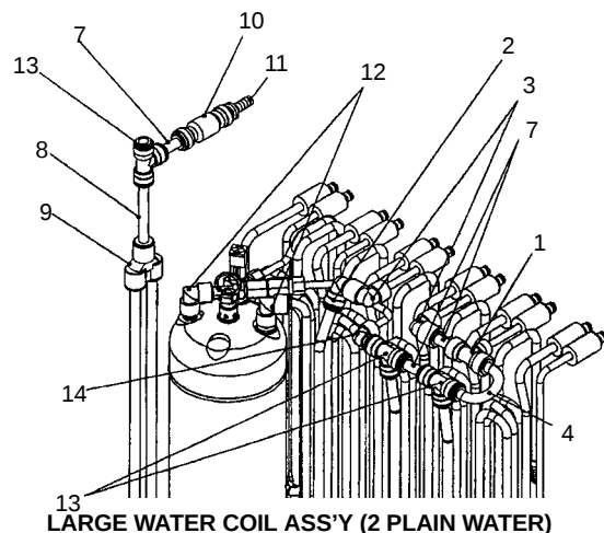
LARGE WATER COIL ASS'Y (2 PLAIN WATER)
