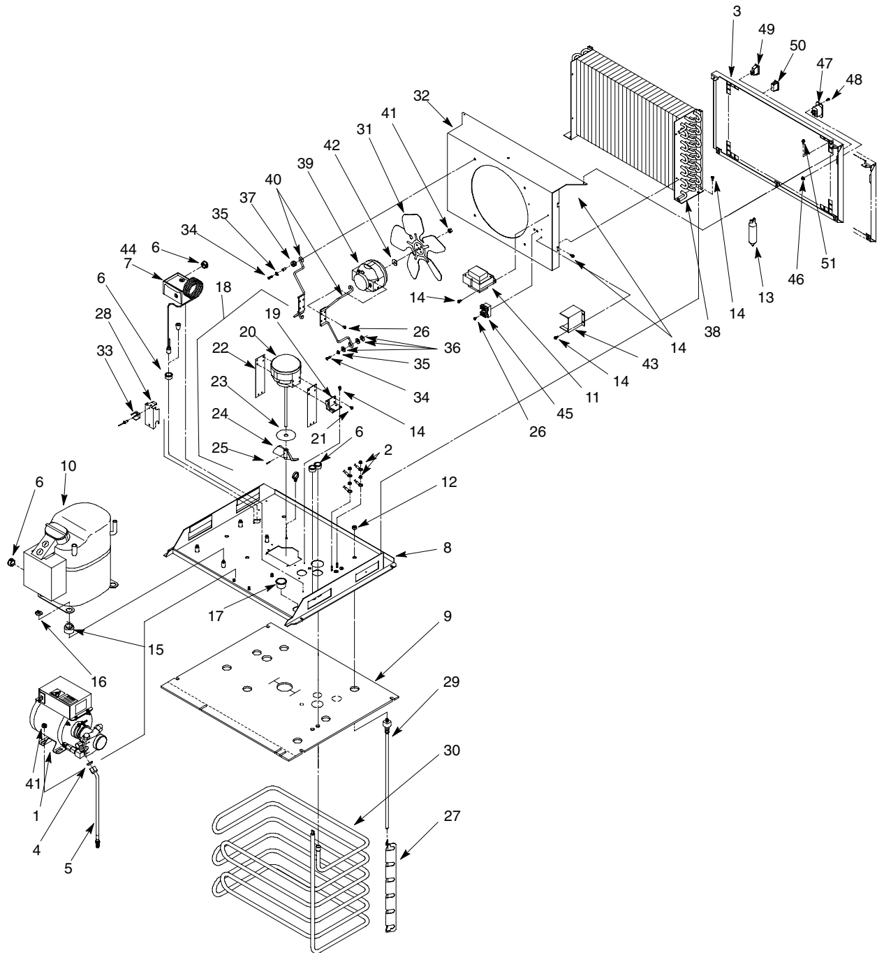
FIGURE 4. VANGUARD 245 REFRIGERATION (COLD CARB) ASSEMBLY
