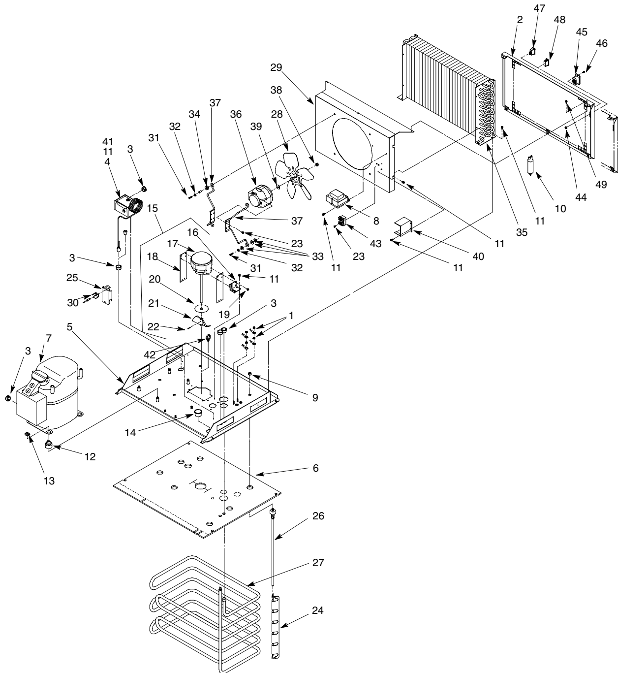
FIGURE 3. VANGUARD 245 REFRIGERATION (REMOTE AND AMBIENT) ASSEMBLY
