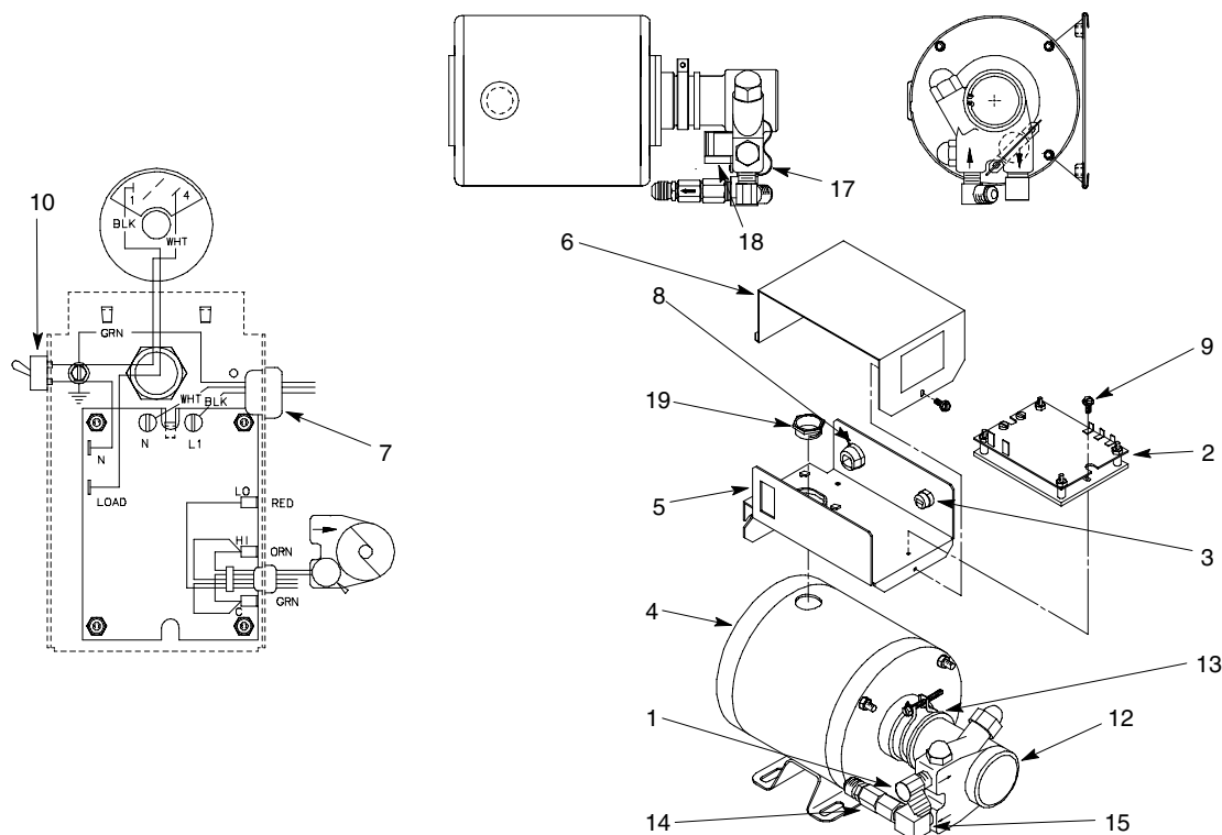
FIGURE 5. PUMP AND MOTOR (COLD CARB) ASSEMBLY
