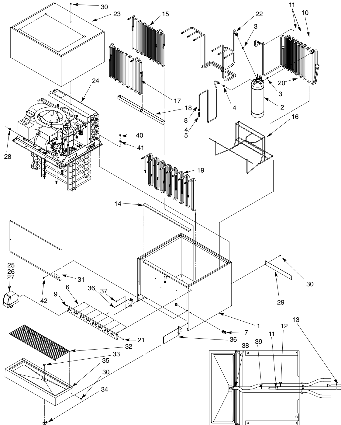
FIGURE 2. VANGUARD 245 POST-MIX DISPENSER (COLD CARB) ASSEMBLY
