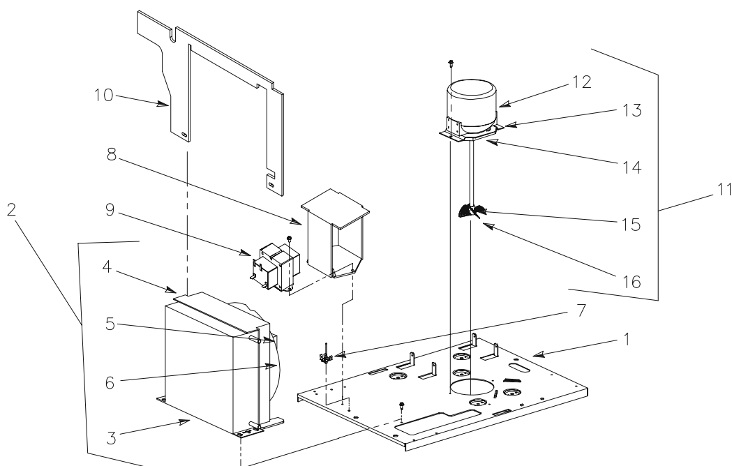
FIGURE 7. CONDENSER COMPONENTS
