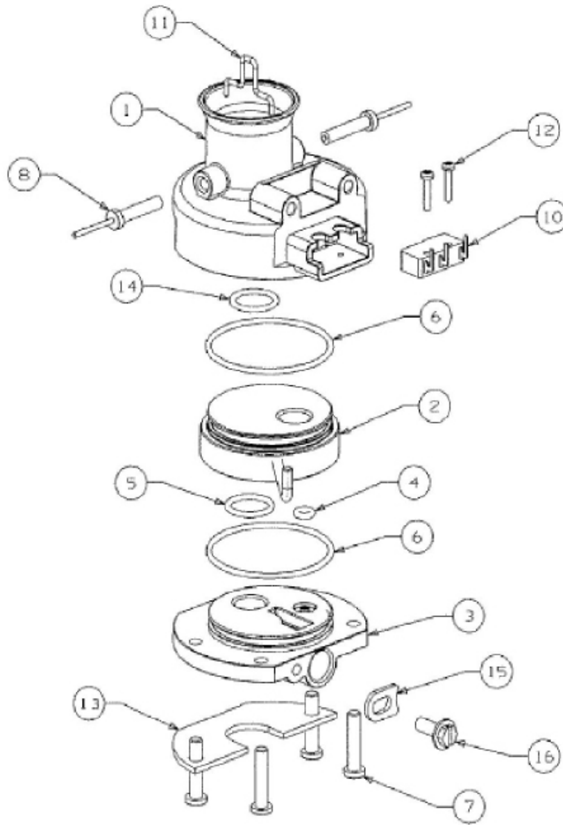
Figure 10. Bottle Adapter Assembly
