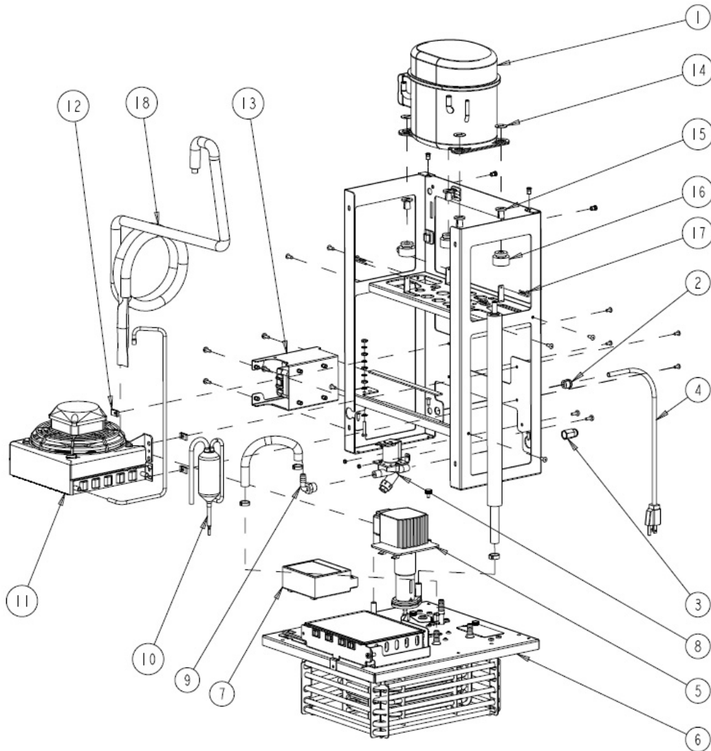
Figure 6. Refrigeration Frame Assembly
