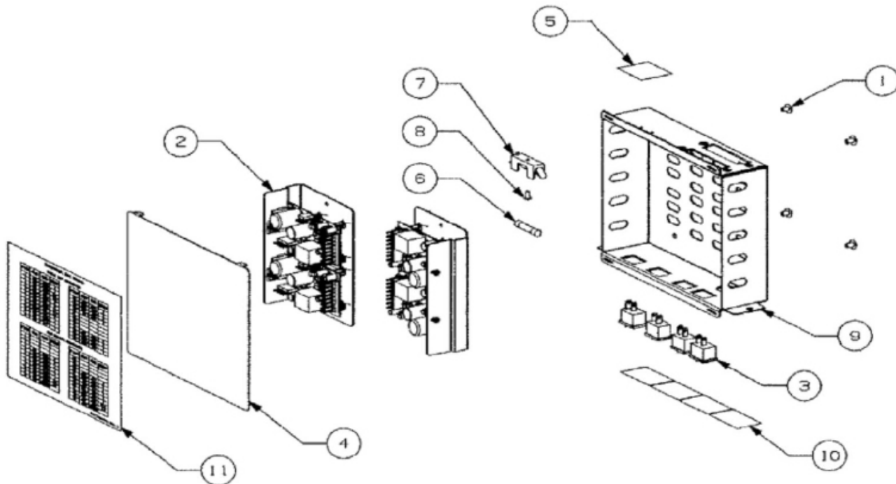
Figure 12. Electrical Box Assembly
