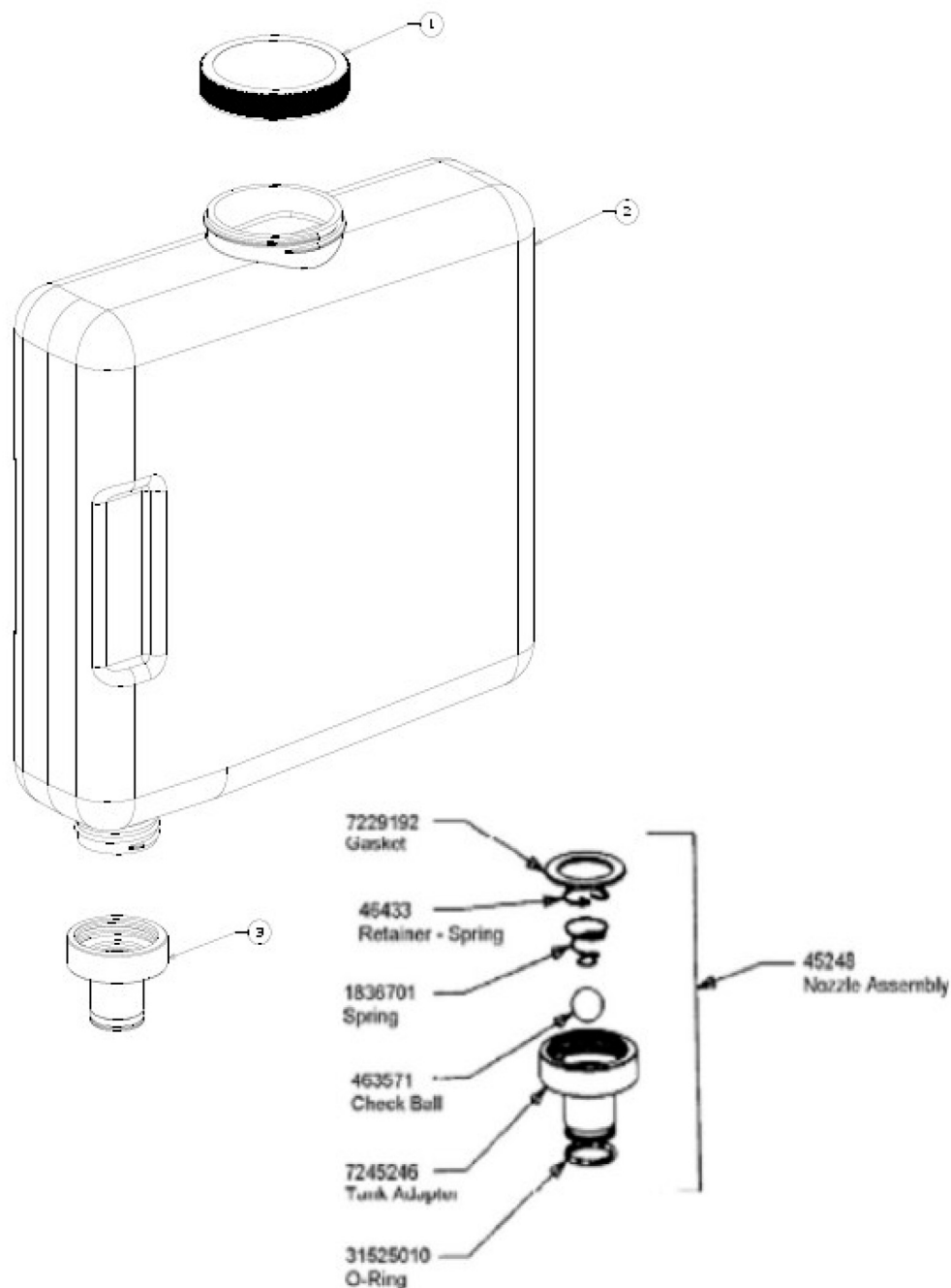
Figure 13. Generic Bottle Assembly
