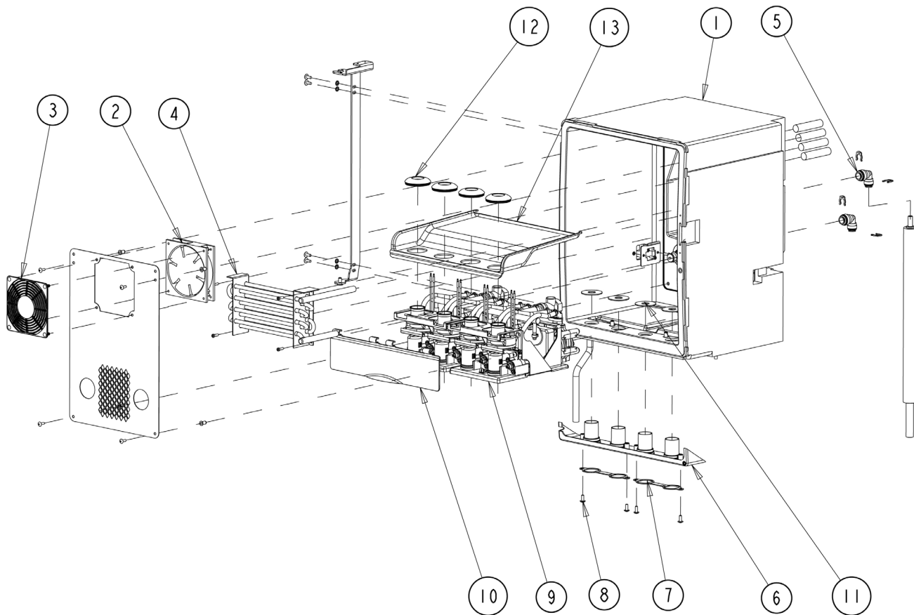
Figure 4. Cabinet Assembly
