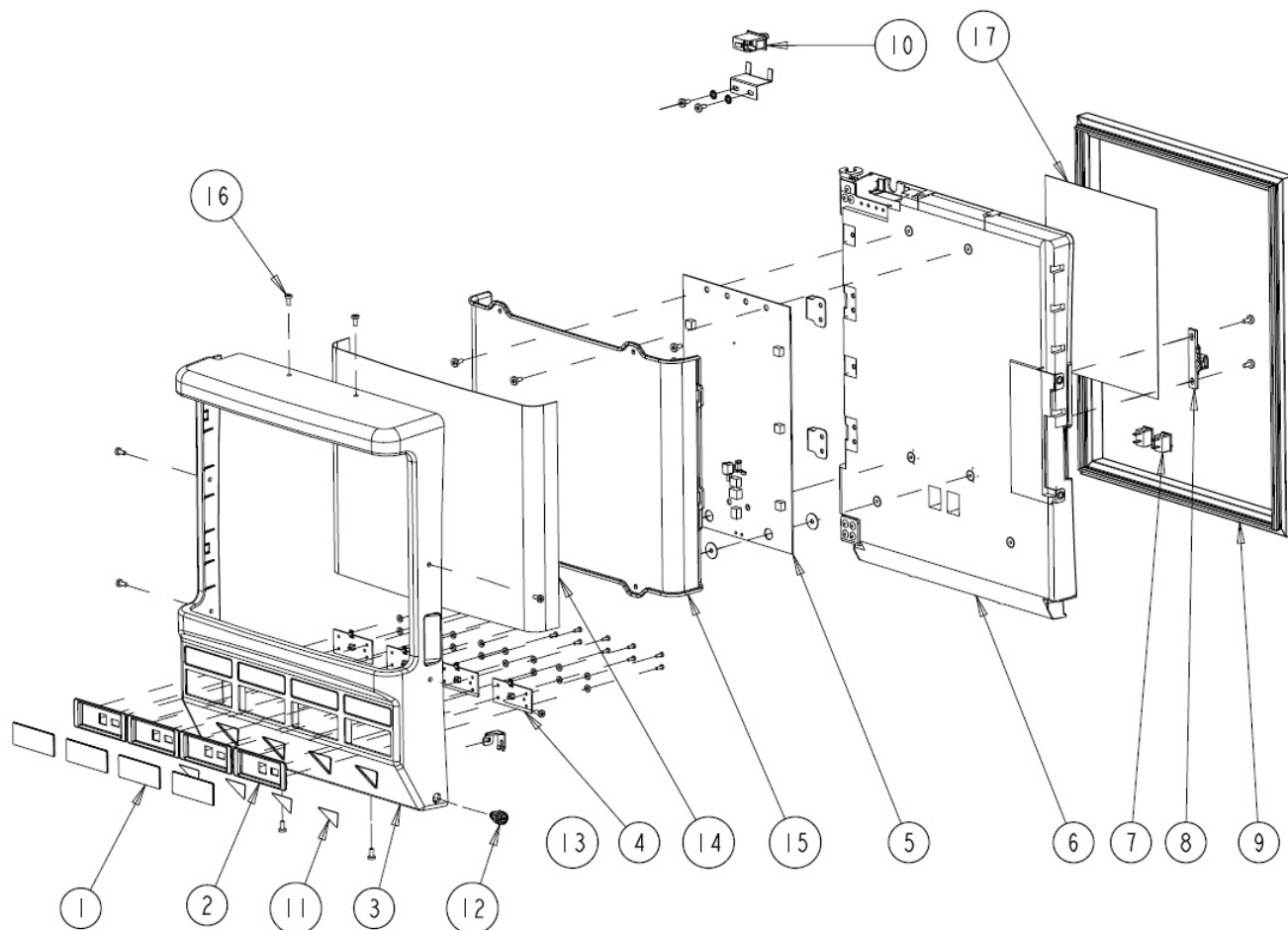
Figure 3. 4000 Door Assembly
