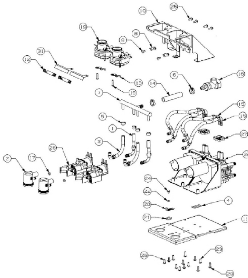
Figure 8. Platform Assembly SLJ
