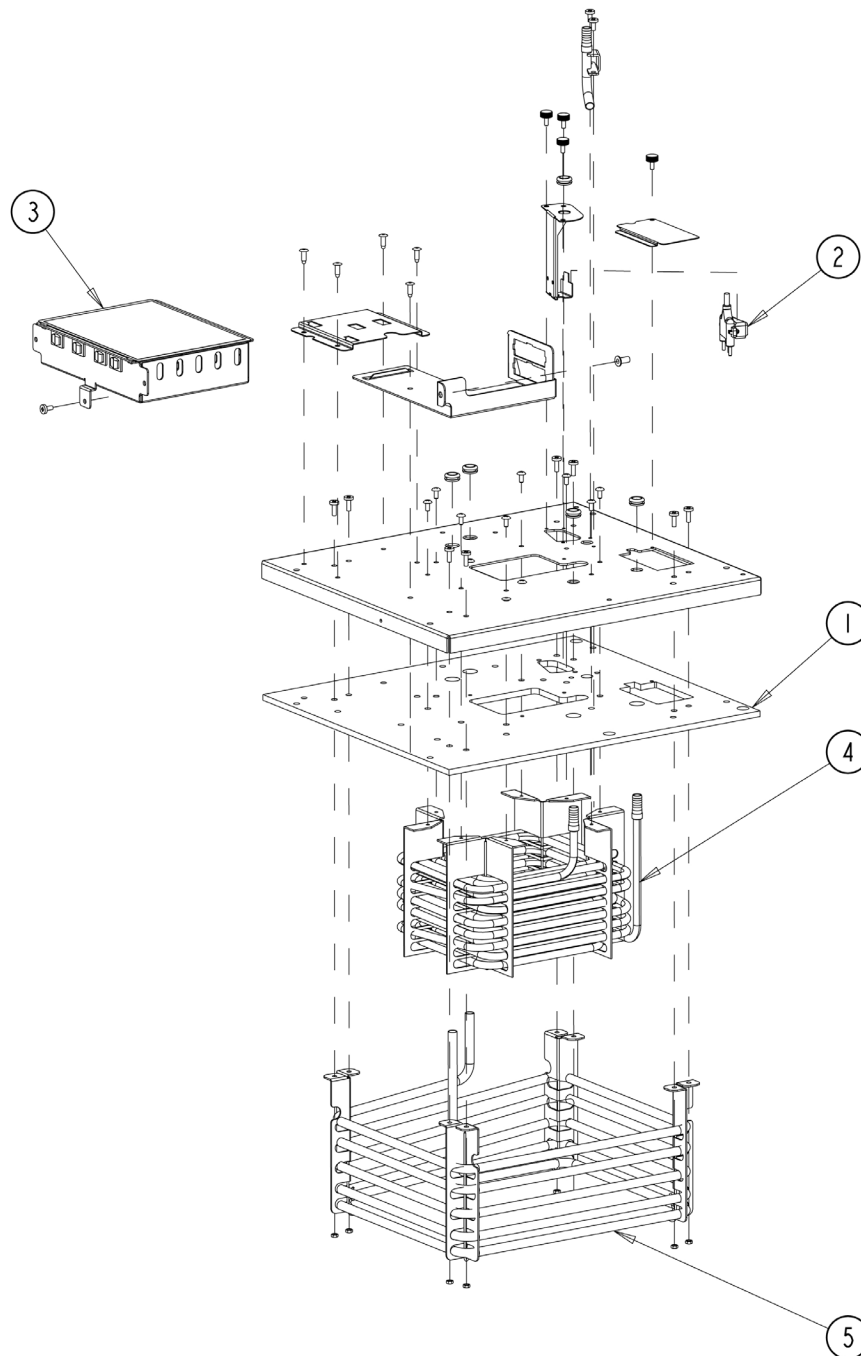
Figure 5. Tank Cover Assembly
