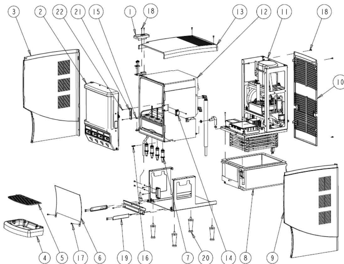
Figure 2. 4FL Final Assembly
