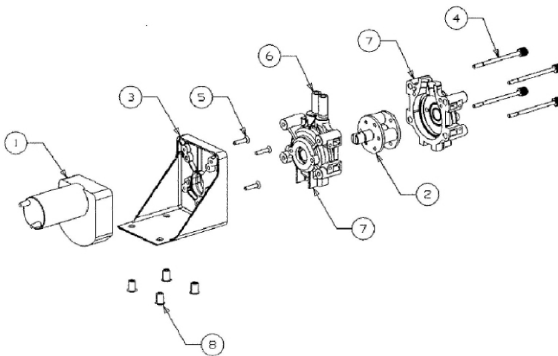
Figure 9. Pump Assembly
