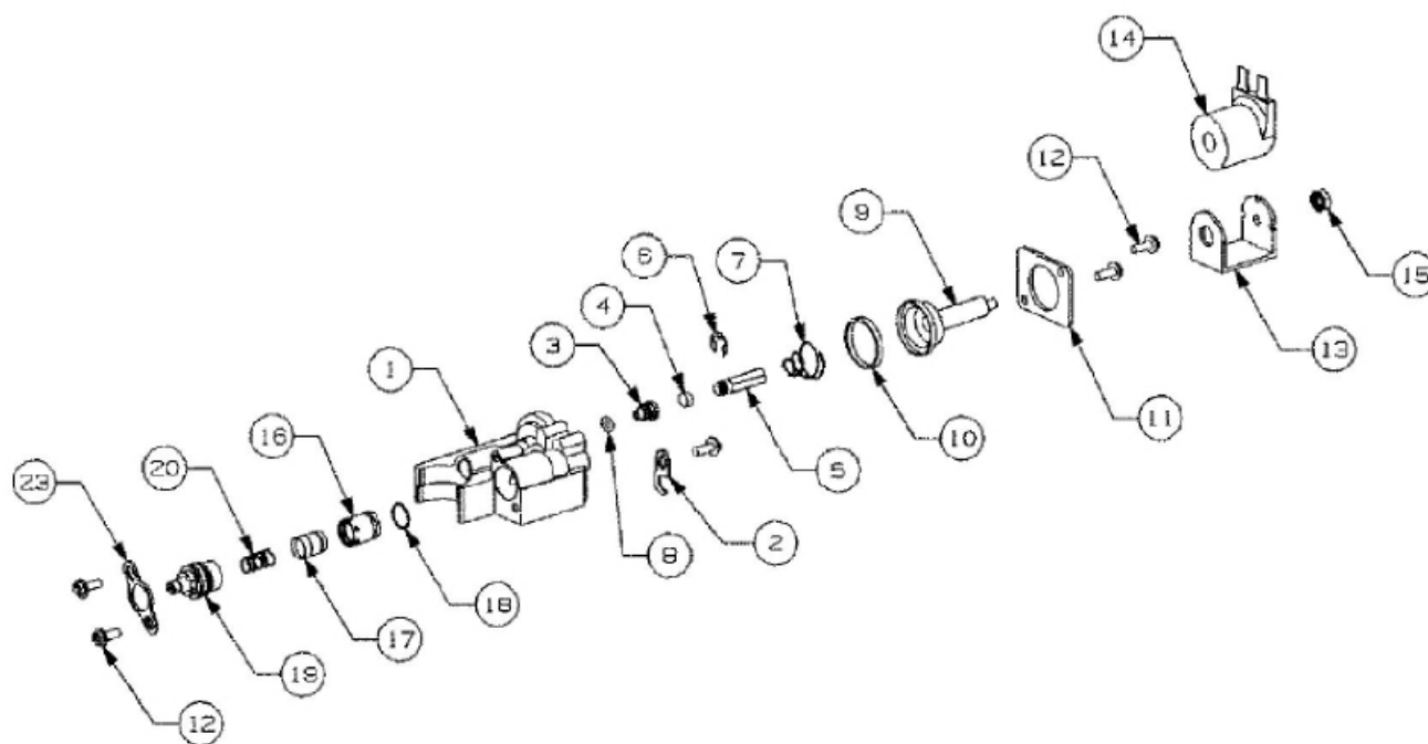
Figure 11. Valve Block Assembly
